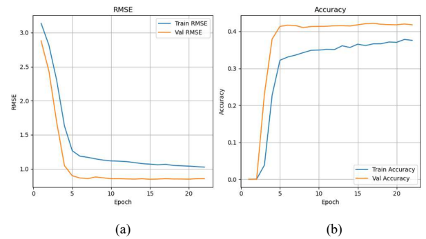
Fig. 3. Training and validation curves over epochs. (a) RMSE. (b) Accuracy.
